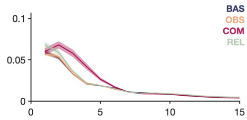
Extended Data Fig. 1 | Power spectra (mean \pm SEM) of LFP recorded during the experimental states in the pooled n=16 electrode pairs that were excluded from analysis as their placement fell wholly or partially across anatomical borders. Compare to Fig. 2b.
