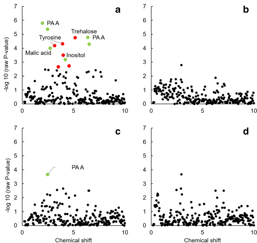
Fig. 2 Negative logarithm of P values of a t -test testing for differences within each bucket (each chemical shift) in the intensity of the signals representing the metabolome of Jacobaea vulgaris grown in 100% sterilized soil and in soil inoculated with soil collected from site A, B, C and D. Red coloured dots represent buckets in which the signal showed a higher intensity and green dots buckets with a lower intensity in plants grown in inoculated soil than in 100% sterilized soil. For signals that
