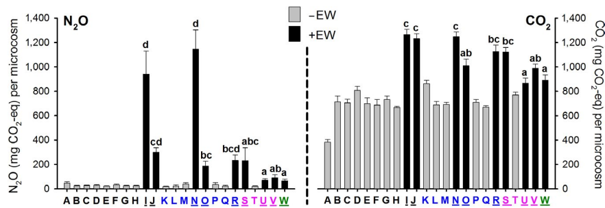
FIGURE 3 Observed cumulative emissions of \text{N}_2\text{O} and \text{CO}_2 after 120 days (in \text{mg CO}_2\text{-eq per microcosm} ). A nonparametric test (Independent-samples Mann-Whitney U test) established the difference in cumulative emissions from treatments with earthworms present (black bars '+EW') compared to treatments without earthworms present (grey bars '-EW'; black bars vs. grey bars: p < .001 for both \text{N}_2\text{O} and \text{CO}_2 ). Lowercase letter denotes differences between treatments with earthworms; any other differences occurring are reported in Table S3. Capital letters placed underneath each bar refer to the species combination given in Table 1. Colours indicate the number of species present: blue = 2 species present, pink = 4 species present and green = 8 species present. Underlined uppercase letters refer to species combinations that include an earthworm species
