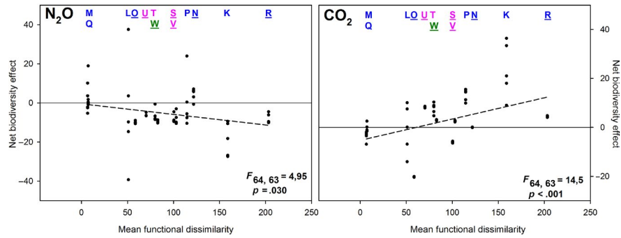
FIGURE 2 Net biodiversity effect on per capita soil-derived emissions of \text{N}_2\text{O} and \text{CO}_2 ( \text{mg N}_2\text{O-N m}^{-2} \text{mg}^{-1} \text{DW} and \text{g CO}_2\text{-C m}^{-2} \text{mg}^{-1} \text{DW} , respectively) in relation to mean functional dissimilarity (sum of effects on \text{NH}_4 , \text{NO}_3 , DOC and pH (Granli & Bøckman, 1994) of species in the community). The 0-line indicates a neutral net biodiversity effect. Each vertical series of dots represent a treatment ( n = 5 replicates per treatment; some dots overlap). For \text{N}_2\text{O} , a significant negative regression between mean functional dissimilarity and the net biodiversity effect (linear regression, F_{64,63} = 4.95 , p = .030 ) indicates that communities with functionally dissimilar species are more likely to have negative net biodiversity effects. For \text{CO}_2 , a significant positive regression between mean functional dissimilarity and the net biodiversity effect (linear regression, F_{64,63} = 14.5 , p < .001 ) indicates that communities with functionally dissimilar species are more likely to have positive biodiversity effects. Uppercase letters at the top of the figure refer to the species combination given in Table 1. Colours indicate the number of species present: blue = 2 species present, pink = 4 species present and green = 8 species present. Underlined uppercase letters refer to species combinations that include an earthworm species
