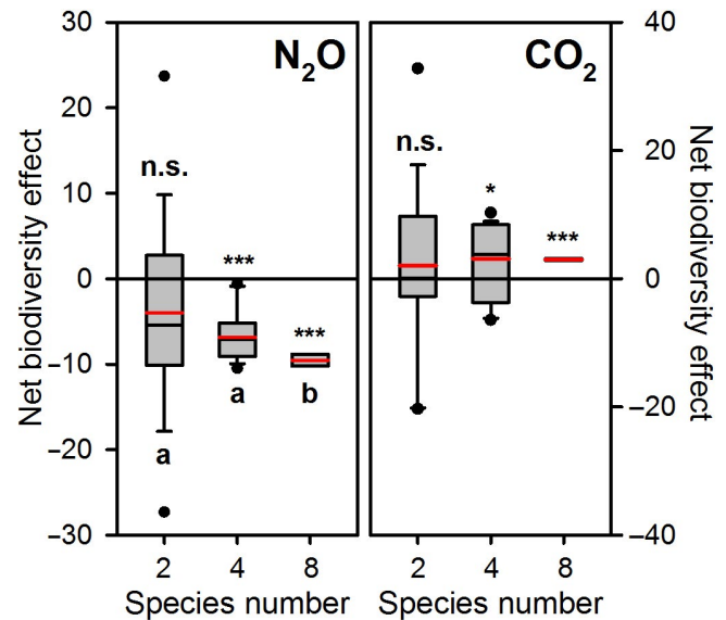
FIGURE 1 Net biodiversity effect on per capita soil-derived emissions of N_2O and CO_2 ( mg\ N_2O-N\ m^{-2}\ mg^{-1}\ DW and g\ CO_2-C\ m^{-2}\ mg^{-1}\ DW , respectively) in relation to species number. The 0-line indicates a neutral net biodiversity effect. Each box plot shows the 5th and 95th percentiles and the mean (red line) of all treatments for two species ( n = 40 ), four species ( n = 20 ) and eight species ( n = 5 ), respectively. Data points that lie outside the 5th and 95th percentiles are shown as dots. For N_2O , significant differences between the two- and eight-species treatments (two-sample t test assuming unequal variances, t statistic = 2.61, p two-tail = .013) and the four- and eight-species treatments (two-sample t test assuming unequal variances, t statistic = 3.70, p two-tail = .001) are indicated by different letters. For CO_2 , there are no significant differences between the two-, four- and eight-species groups. For both N_2O and CO_2 , the four- and eight-species groups are significantly different from the constant 0 (established by a one-sample t test); levels of significance are * <.05 ; ** <.01 ; *** <.001 ; ns = not significant
