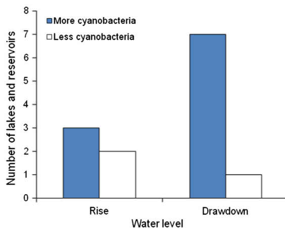
Fig. 1 Number of lakes and reservoirs with more or less cyanobacteria in response to different types of water-level fluctuation. The response of each water body is documented in Table 1
