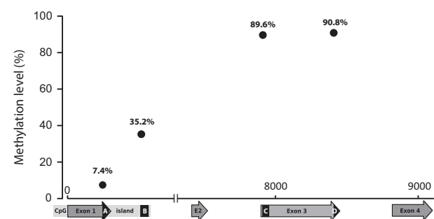
Fig. 2 The mean methylation levels in blood tissue. The increase in methylation towards the 3' end of DRD4 is shown with the position of the assay in the gene on the x -axis. The four pyrosequence assay positions (A, B, C and D; black box with white letters), exons (dark grey arrows) and CpG island (light grey box) are shown on the x -axis with the numbers denoting base pairs starting from the transcription start site.
