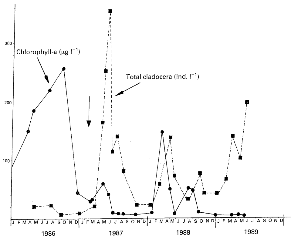
Fig. 2 — The concentrations of chlorophyll-a and cladocera in Lake Zwemlust before and after ecological management.
