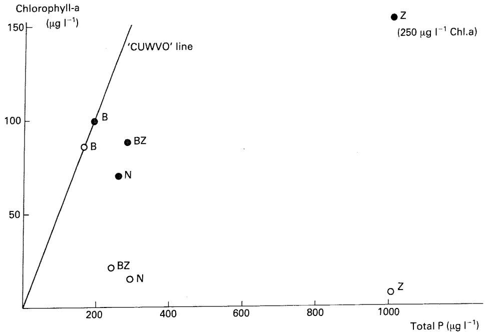
Fig. 5—The relation between chlorophyll-a and total P. The so-called 'CUWVO' line represents the maximum concentration of chlorophyll-a at different total P concentrations, based on a large number of observations in Dutch inland waters (CUWVO 1988). The values of the lakes are given before (●) and after ecological management (○). B=Lake Breukeleveen; BZ=Lake Bleiswijkse Zoom; N=Lake Noorddiep; Z=Lake Zwemlust.
