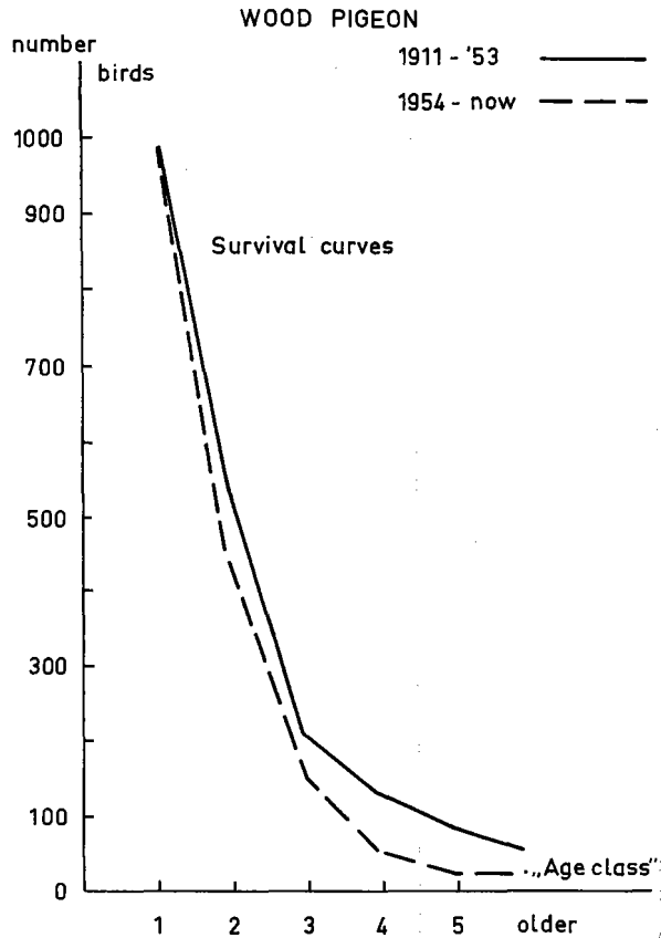
FIGURE 1. Survival curves for the periods 1911-1953 and 1954-1962, based on 113 and 66 recoveries, respectively, of Woodpigeons ringed in the Netherlands. The data used for the construction of the curves have been given in Table 1.
