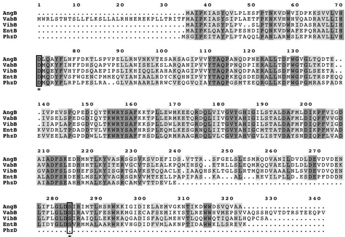
Fig. 3 Multiple sequence alignment of isochorismate lyase enzymes. All the proteins in this alignment except PhzD participate in DHBA biosynthesis as well as in siderophore biosynthesis. PhzD possesses only the ICL domain and it is involved in the biosynthesis of phenazine. The identical
