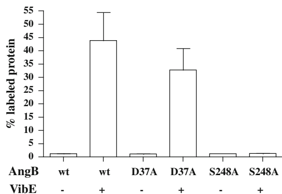
Fig. 6 In vitro salicylation reaction with purified wild type and mutant AngB proteins. The percentage of ArCP domain labeled with [ ^{14} C]-salicylate is shown with each bar calculated from the mean of three independent experiments in which the same amounts of proteins and substrate were used. As controls each AngB protein was incubated without the adenylating enzyme VibE. The means for the wild type and the D37A mutant AngB proteins are not significantly different when compared by the t -test at P \leq 0.05 ( P = 0.45 ). The error bars indicate the standard error of the mean of the results from replicate samples. wt, wild type AngB; D37A, D37A mutant of AngB; S248A, S248A mutant of AngB
