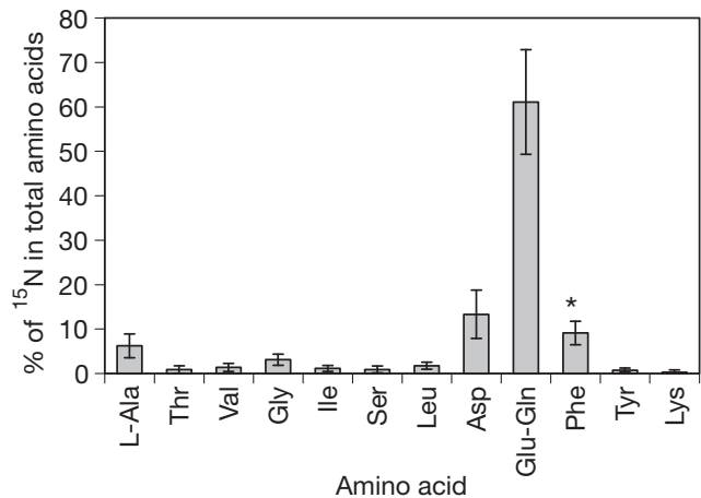
Fig. 6. Elysia viridis . Relative incorporation of 15 N from 15 N-ammonium in different hydrolyzable amino acids, for green individuals incubated under both light and dark conditions (pooled data, since labeling patterns were similar, n = 4). Note that during hydrolysis, Gln is converted to Glu, so the Glu-Gln peak refers to both Glu and Gln. *Partial overlap of Phe with the Glu-Gln peak occurs, and part of the 15 N reported for Phe may be due to high labeling of Glu-Gln. Error bars: 1 SD
