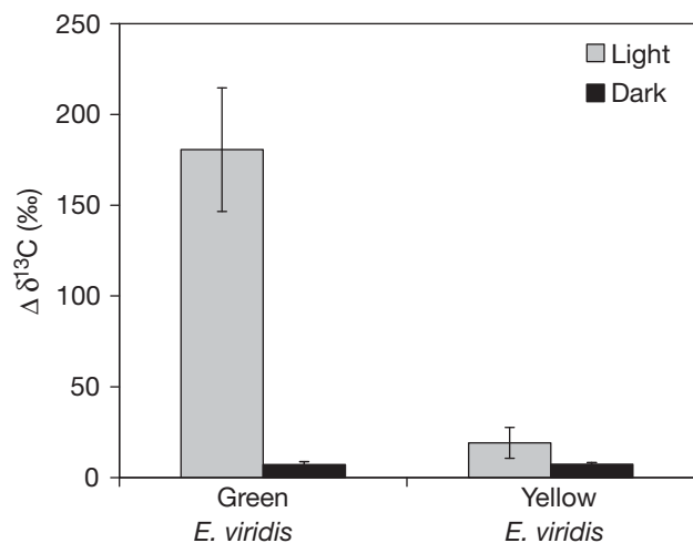
Fig. 3. Elysia viridis . Enrichment in ^{13}\text{C} for green and yellow individuals after exposure to artificial seawater spiked with 1\text{ mmol l}^{-1} ^{13}\text{C} -bicarbonate for 30 h in either light or dark conditions. Error bars: 1 SD ( n = 3 for green individuals, n = 2 for yellow individuals)
