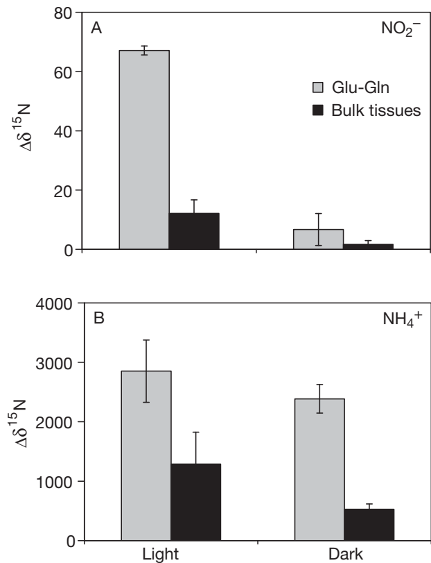
Fig. 5. Elysia viridis . Enrichment in 15 N in hydrolyzable glutamine/glutamate and bulk tissues for green individuals exposed to (A) 15 N-labeled nitrite or (B) 15 N-labeled ammonium under light and dark conditions. Error bars: 1 SD
