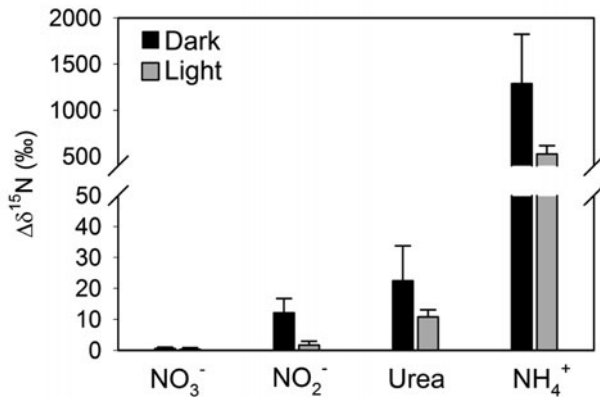
Fig. 4. Elysia viridis . 15 N labeling of green individuals after exposure to artificial seawater spiked with either 40 μmol l -1 K 15 NO 2 , 40 μmol l -1 K 15 NO 3 , 40 μmol l -1 15 NH 4 Cl, or 20 μmol l -1 CO( 15 NH 2 ) 2 for 20 h in either light or dark conditions. Error bars: 1 SD (n = 3)
