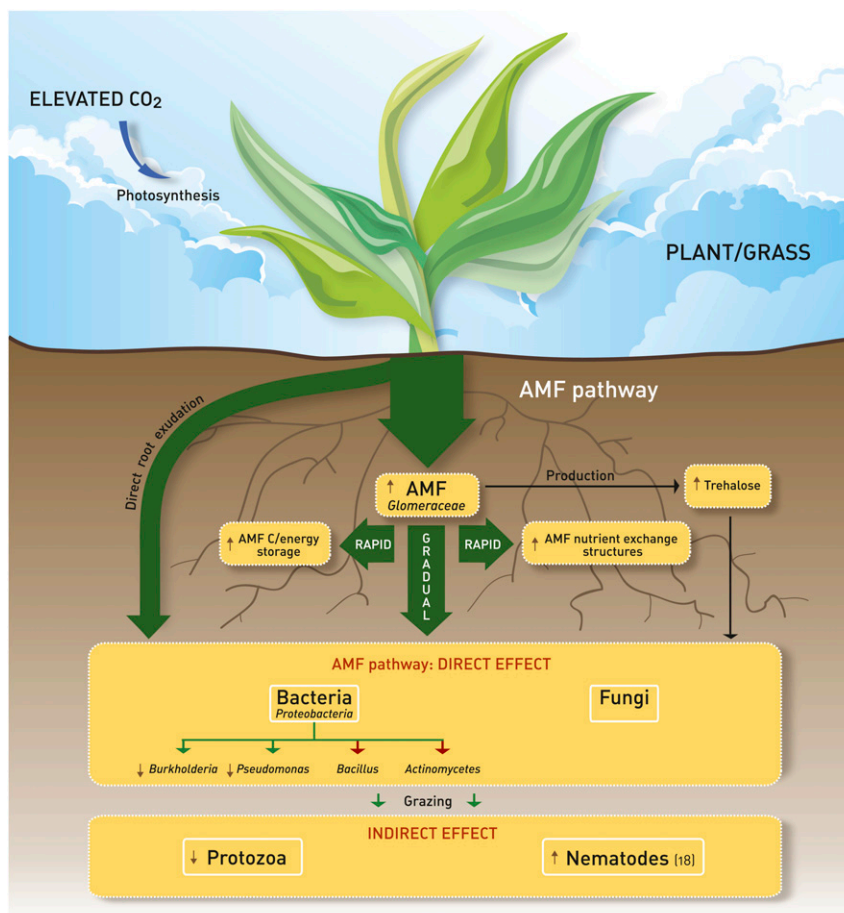
Fig. 4. Conceptual model of C flow in mycorrhizal plant–soil systems summarizing the observed effects of elevated \text{CO}_2 atmospheric concentrations on soil communities. Brown arrows indicate increases and decreases in the respective community sizes, as determined by real-time PCR and lipid analyses from this study and ref. 18, as well as changes in community structure and carbon flow. Absence of an arrow indicates no significant change in the community size or structure. Red arrows indicate no effect of increased C availability because of elevated \text{CO}_2 on the Actinomycetes spp. and Bacillus spp. communities. The mechanism and magnitude of the C flow along the soil–food web are indicated by the green arrows. Effects on nematodes are based on ref. 18.
