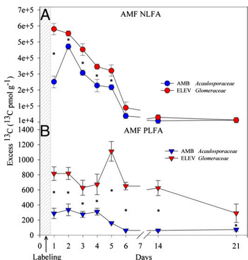
Fig. 1. ^{13}\text{C} enrichment in the AMF signatures 16:1 05 determined in F. rubra rhizosphere soil for NFLA (circles; A) and PLFA (triangles; B) at ambient \text{CO}_2 (blue) and elevated \text{CO}_2 (red). The given AMF families, Acaulosporaceae and Glomeraceae , denote the affiliations of the 18S rRNA gene fragments recovered from the ^{13}\text{C} -labeled RNA fractions by RNA-SIP at ambient \text{CO}_2 and elevated \text{CO}_2 , respectively. Asterisks designate significant differences ( P < 0.001 ) between \text{CO}_2 concentrations. The values given are the average of biological replicates, and errors represent the standard error.
