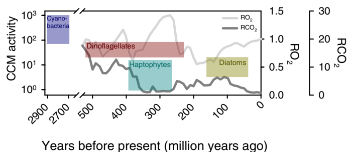
Fig. 1. The evolutionary origin of phytoplankton groups and associated CCM activities. The gray lines describe changes in Phanerozoic atmospheric O 2 and CO 2 concentrations relative to the present (i.e. RO 2 and RCO 2 ; Berner 2006), and the colored boxes denote the CCM activities as a function of the evolutionary origin of four key phytoplankton groups. The CCM activity expresses the concentration factor of intracellular over extracellular C i concentration at present-day conditions for cyanobacteria (blue; Badger and Andrews 1982, Volokita et al. 1984), dinoflagellates (red), haptophytes (cyan), and diatoms (yellow; Badger et al. 1998). The evolutionary origin is based on fossil records of cyanobacteria (Nisbet et al. 2007), fossil records and biomarkers of dinoflagellates (Fensome et al. 1996; Moldowan and Talyzina 1998), and molecular clock analyses of haptophytes and diatoms (Young et al. 2012).
